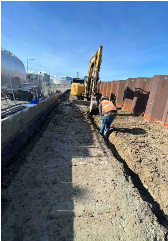
Levee retaining wall under construction
